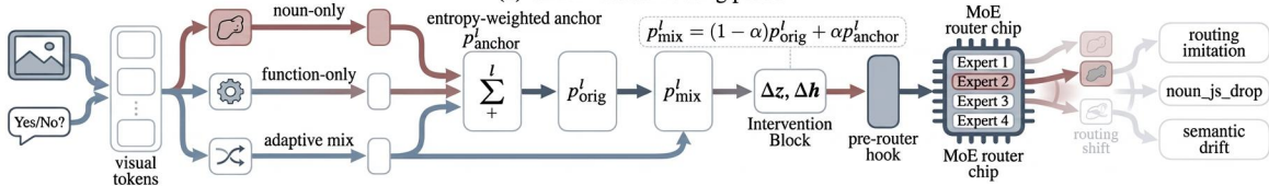
(a) CMRD causal routing probe
